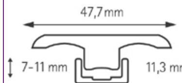
T-list
