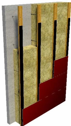
Figure 1: REDAir® FLEX system overview. The wall and cladding panels are not part of the REDAir® product offering and included only for illustration purposes.
